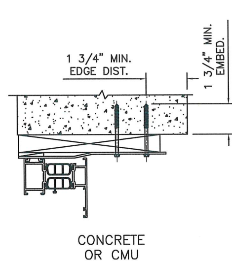
TYPICAL ANCHOR CONDITIONS WITH OPTIONAL WOOD BUCKS (1x MAX)
